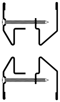
LT-B3 13/16" Glazing Pocket for 5/8" to 3/4" Glass
