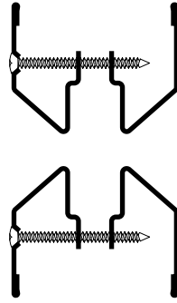
LT-B2 9/16" Glazing Pocket for 3/8" to 1/2" Glass
