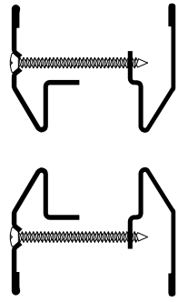
LT-B4 1 1/16" Glazing Pocket for 7/8" to 1" Glass
