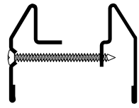
LT-B4 1 1/16" Glazing Pocket for 7/8" to 1" Glass
