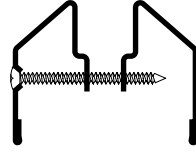
LT-B2 9/16" Glazing Pocket for 3/8" to 1/2" Glass
