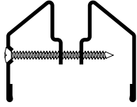
LT-B1 3/8" Glazing Pocket for 1/4" Glass
