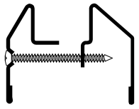
LT-B3 13/16" Glazing Pocket for 5/8" to 3/4" Glass
